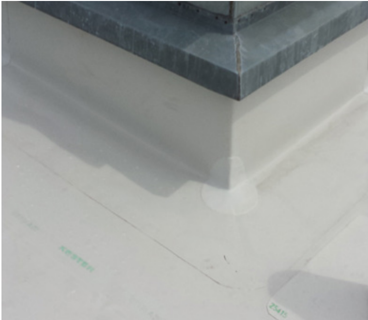
Junctions to right-angled penetrations
