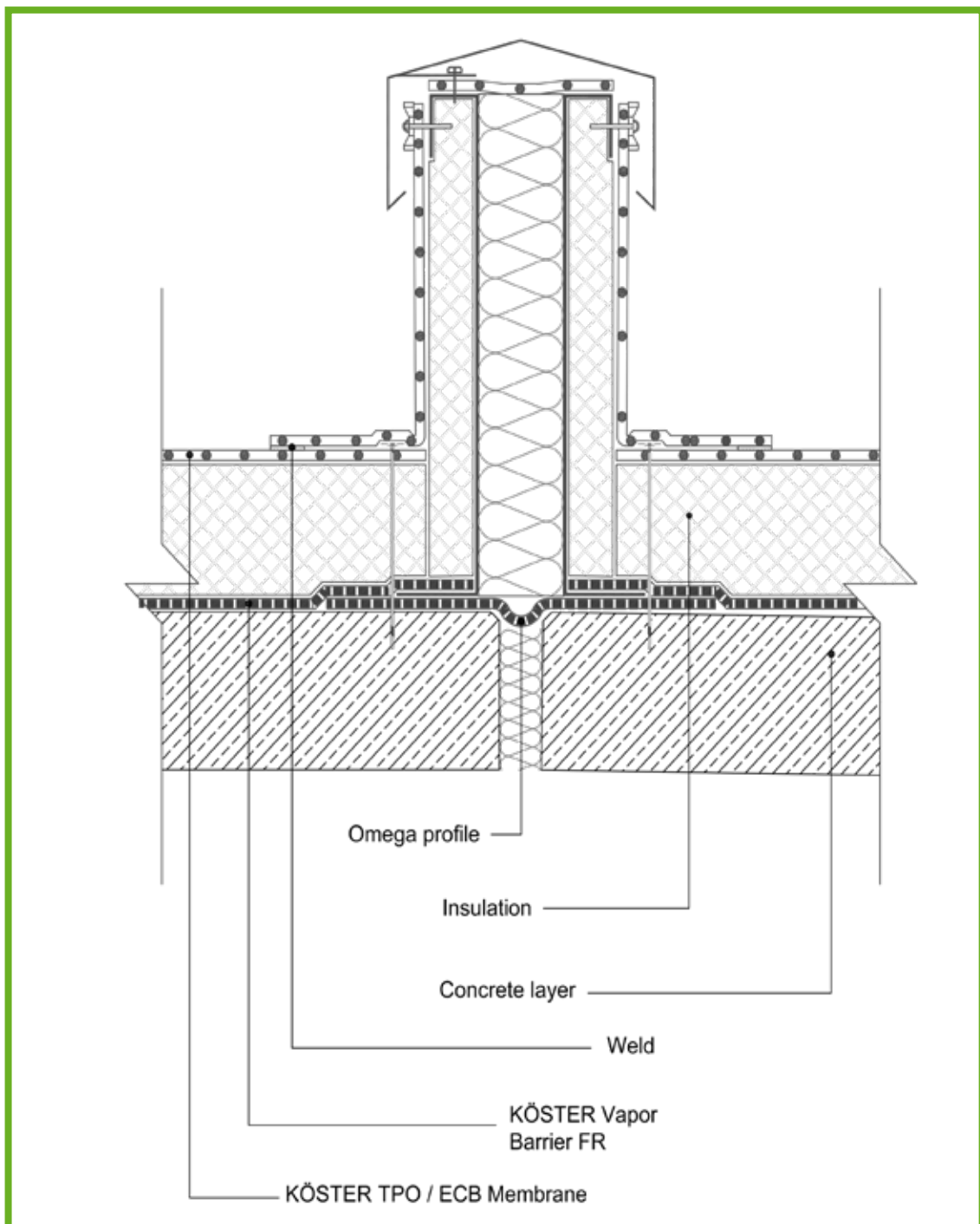
Joint type II
