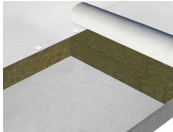
Mechanically fastened installation
