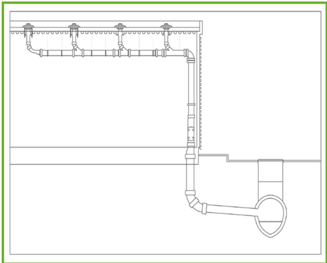
Pressurized roof drainage
