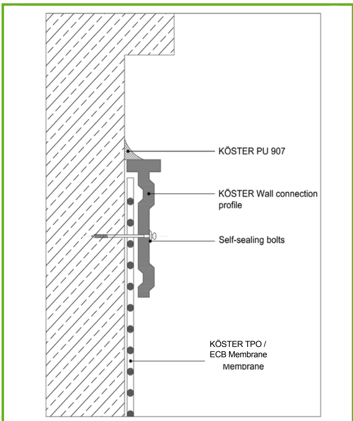
Upper transition with clamping profile
