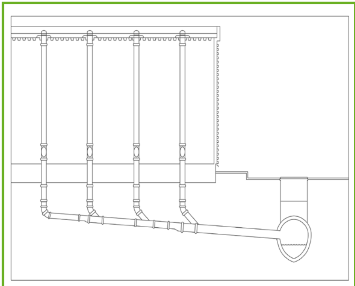
Gravity roof drainage
